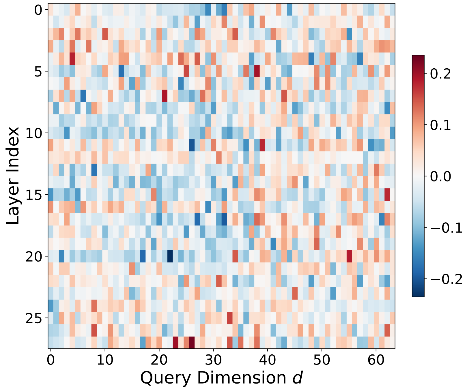
(a) Learned Layer Bias
