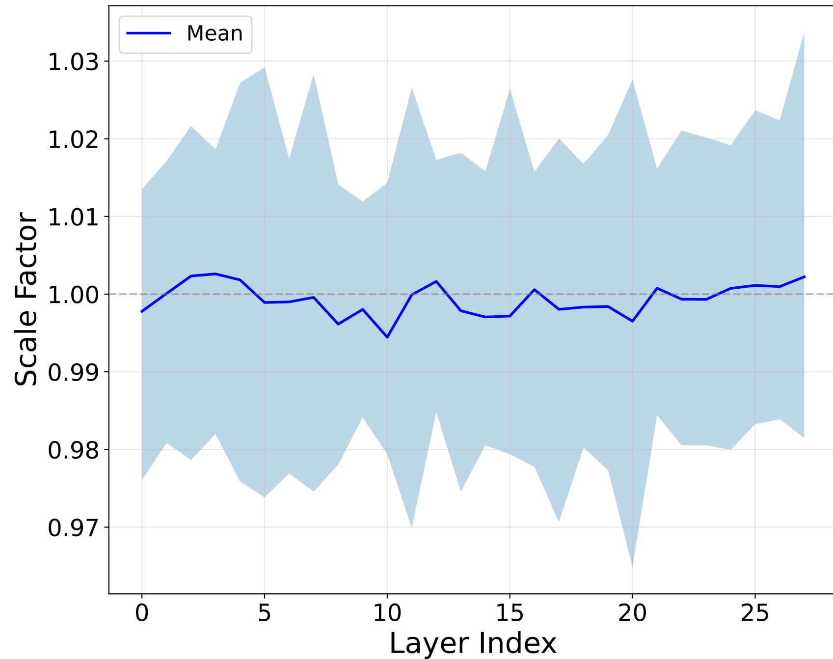
(b) Modulation Range per Layer ( \alpha=0.3 )
