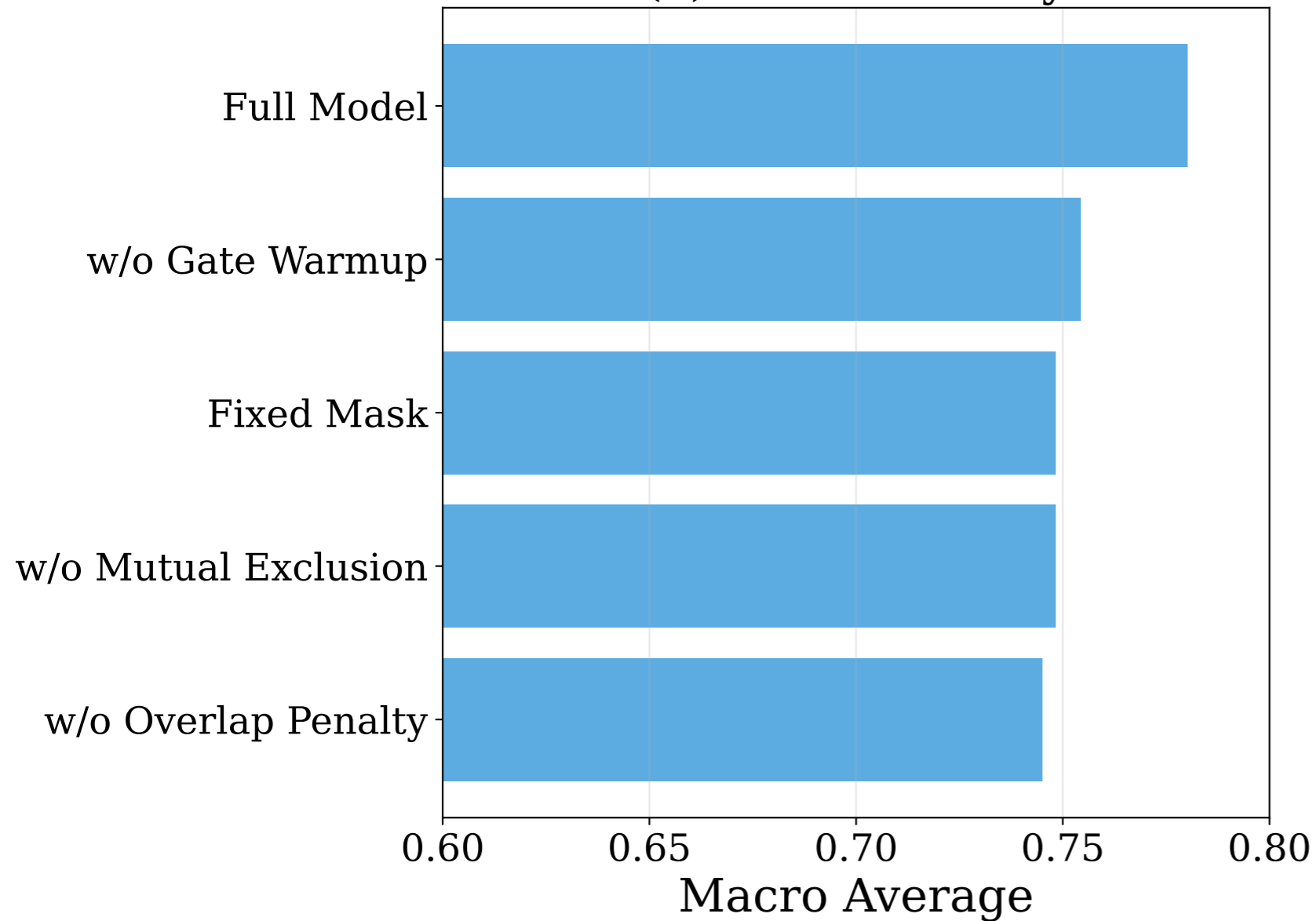
(a) Ablation Study
