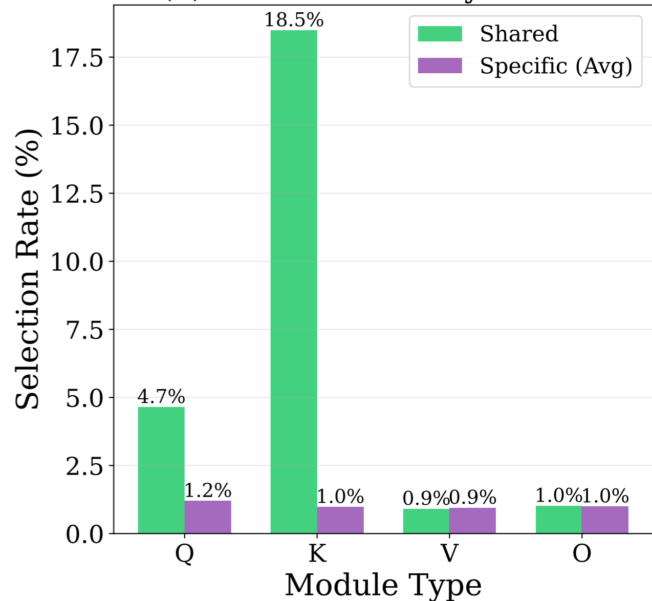
(b) Selection Rate by Module
