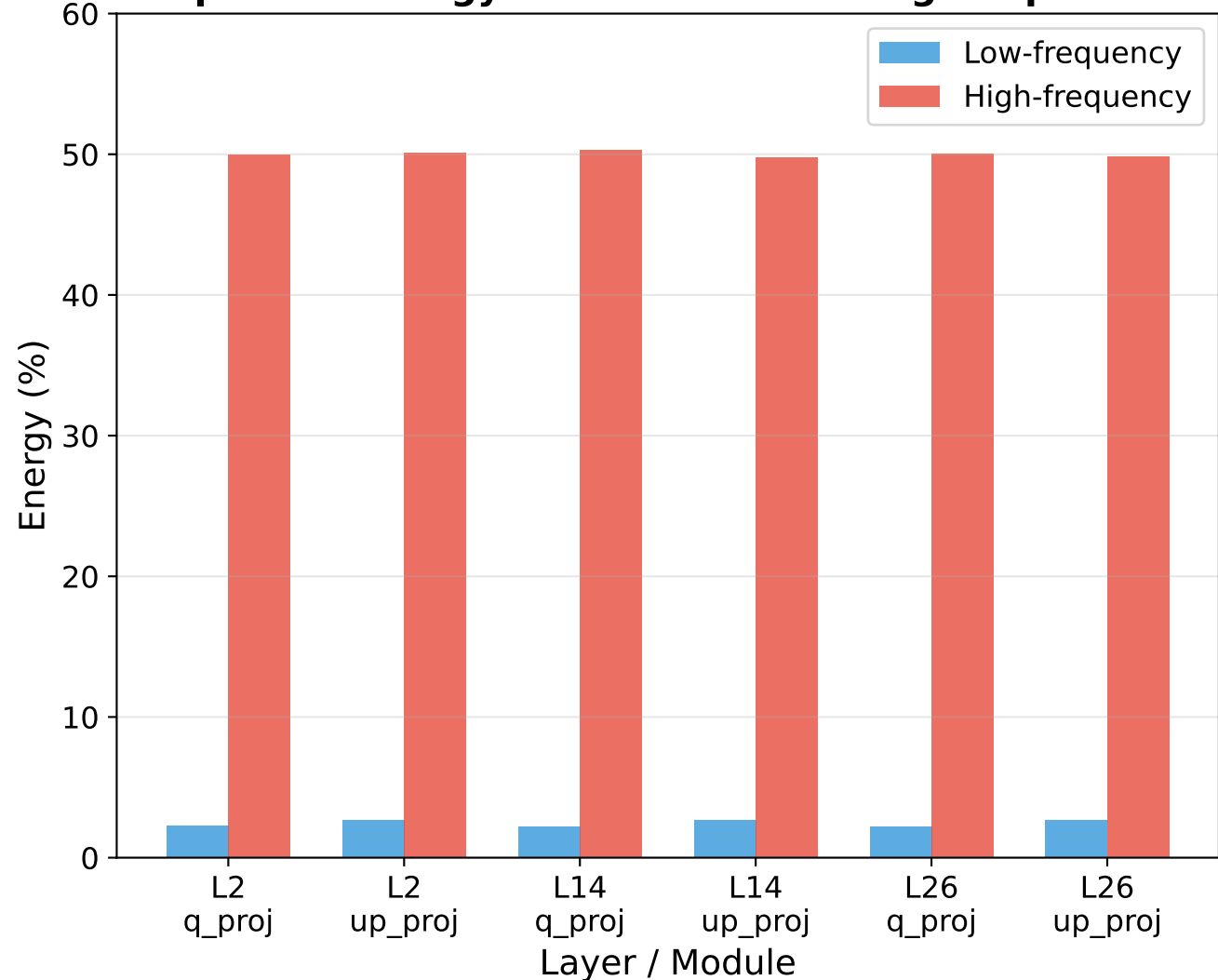
Spectral Energy Distribution of Weight Updates
