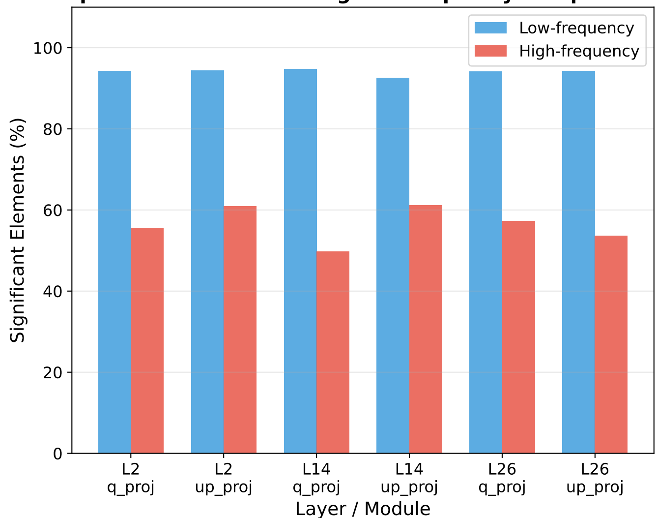
Spatial Influence Coverage of Frequency Components
