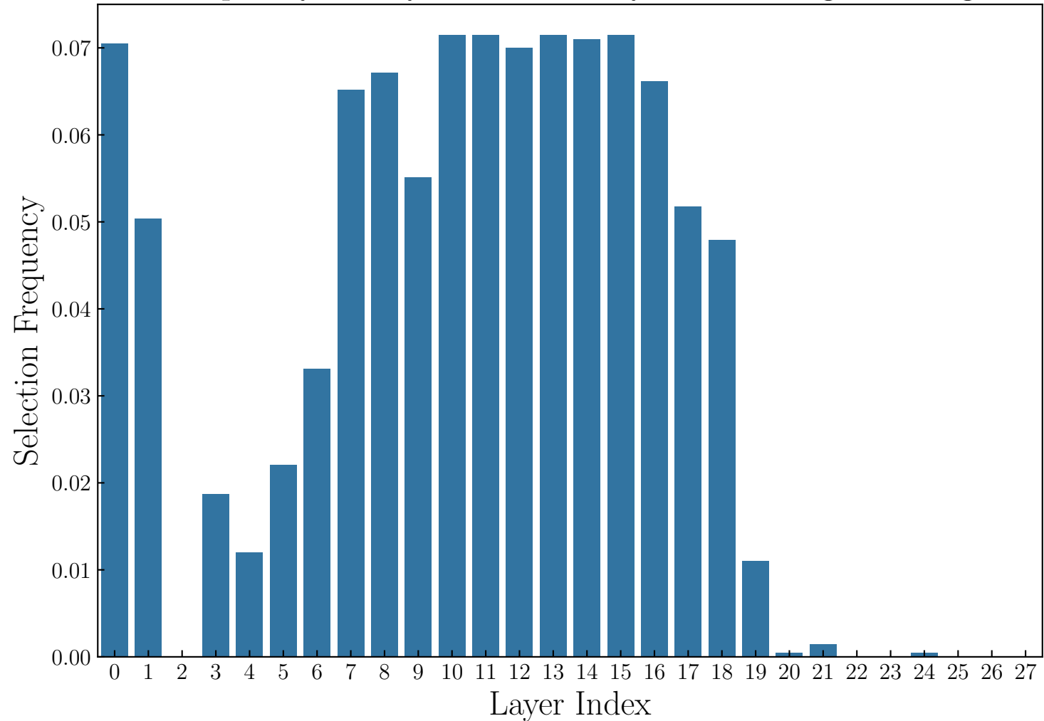
Frequency of Layers Selected by DLS during Training
