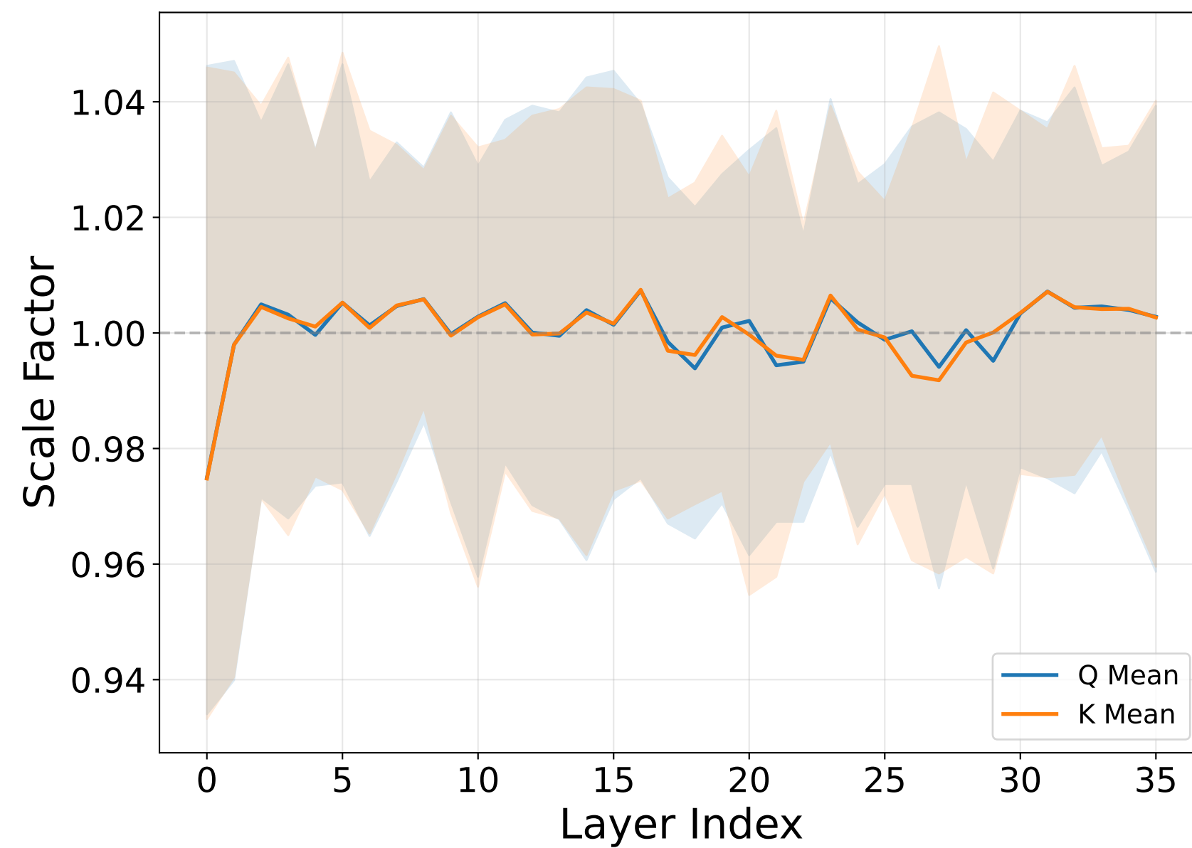
(e) Qwen3 Math ( \alpha=0.3 )
