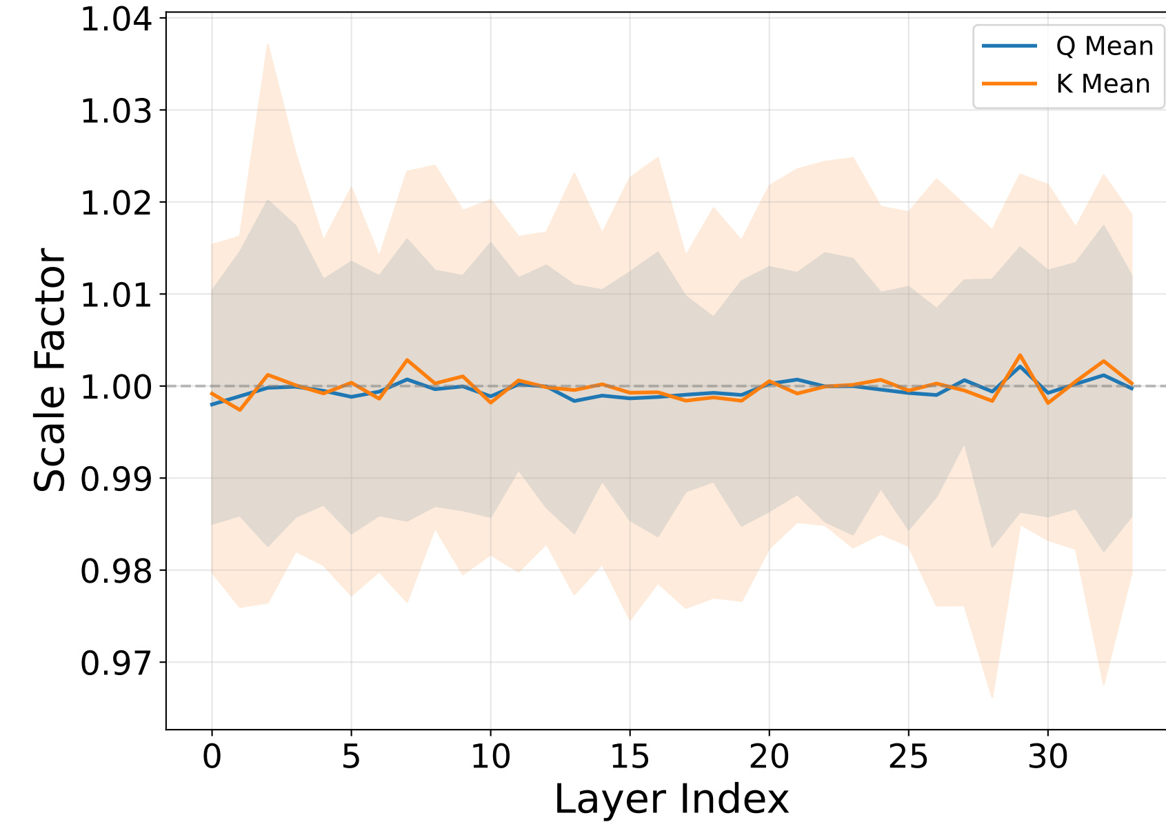
(f) Gemma3 Math ( \alpha=0.3 )
