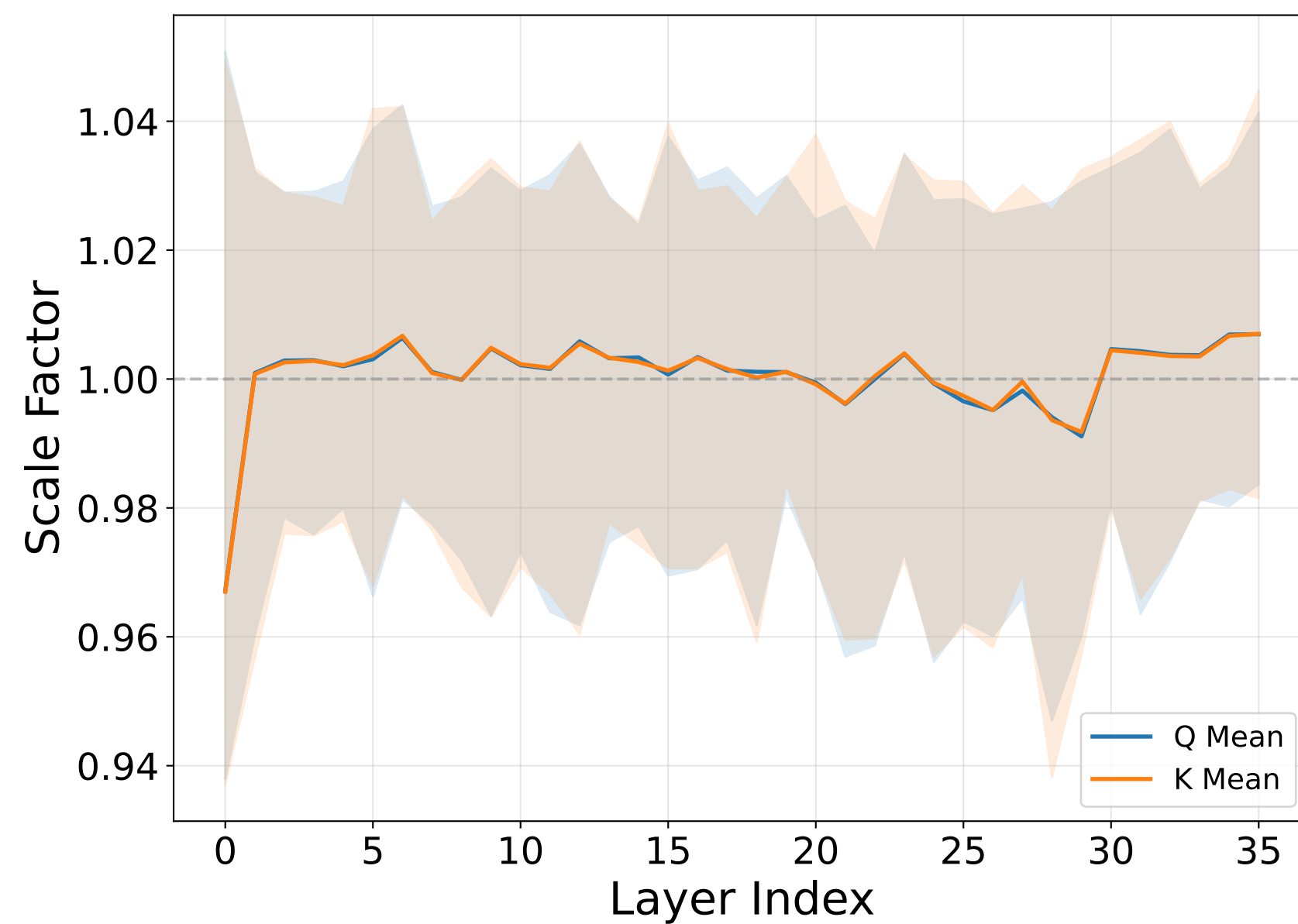
(e) Qwen3 Math ( \alpha=0.3 )
