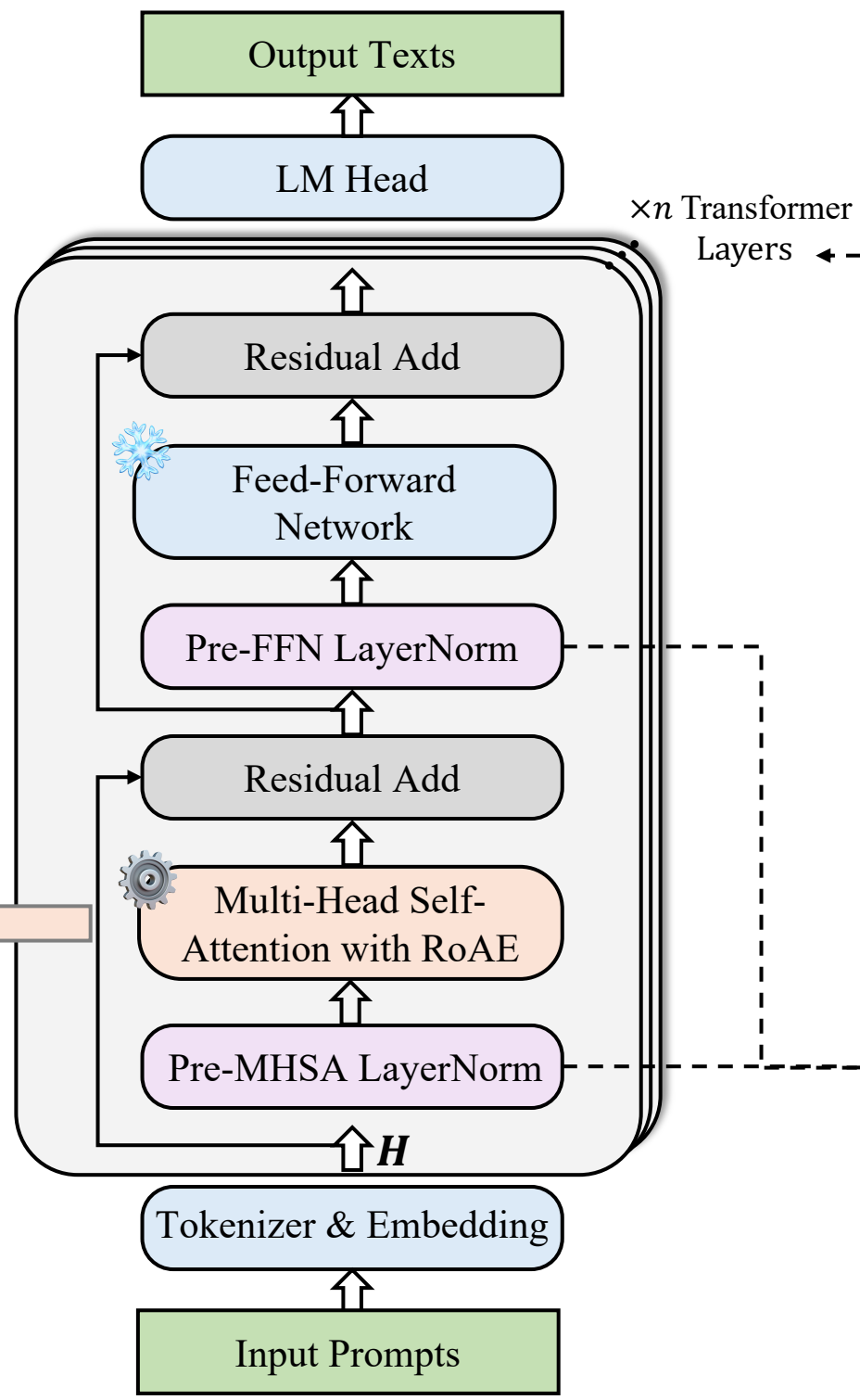
Overall Framework of RoSA
