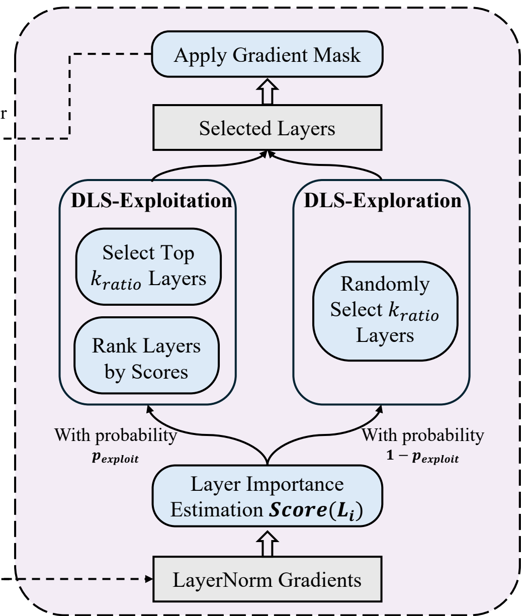
DLS Strategy with LayerNorm Gradients
