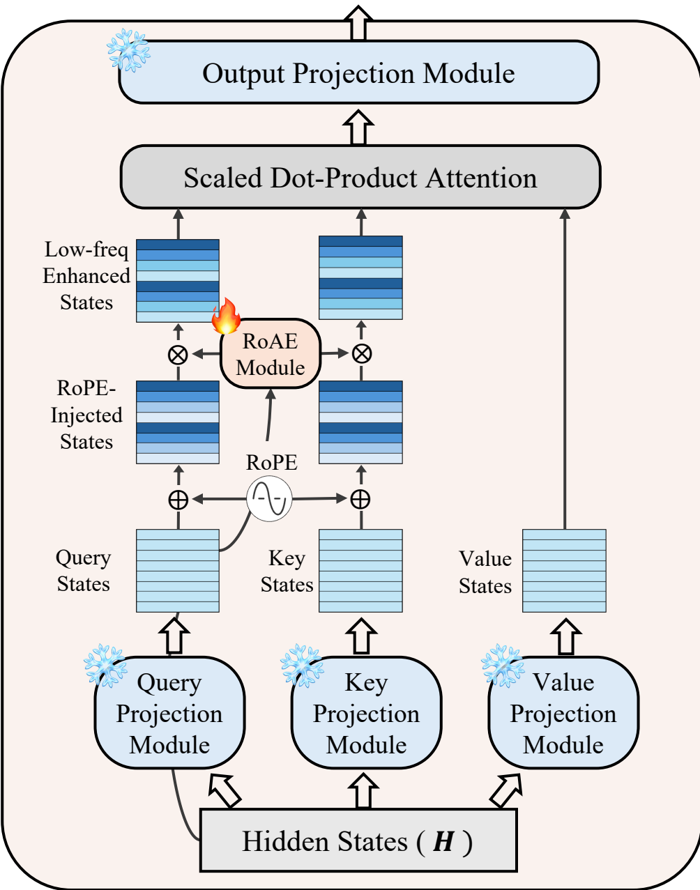
RoAE Mechanism in MHA
