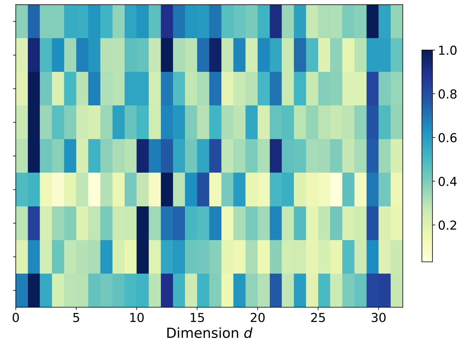
Layer 12, Head 2
