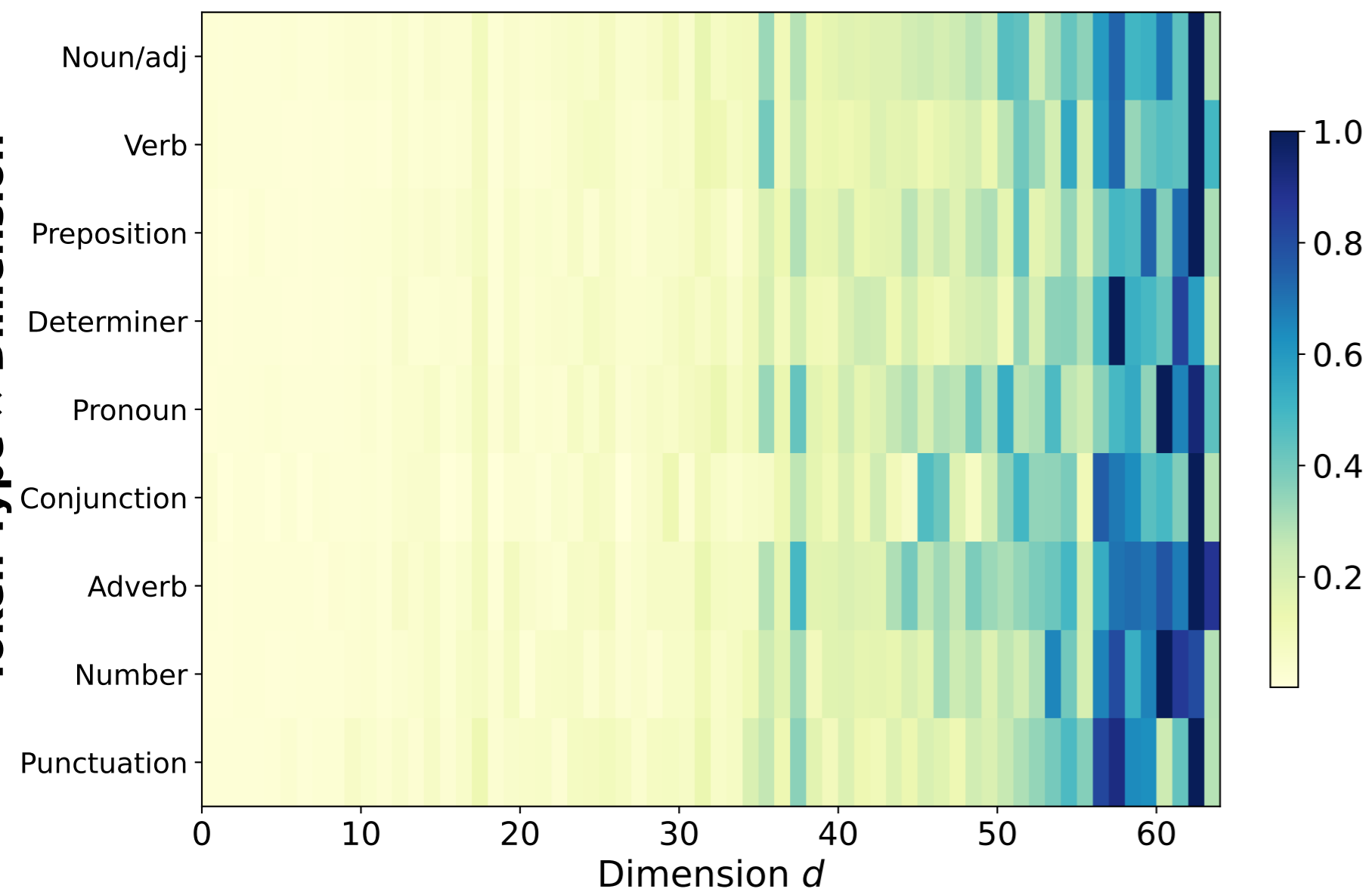
Layer 14, Head 2
