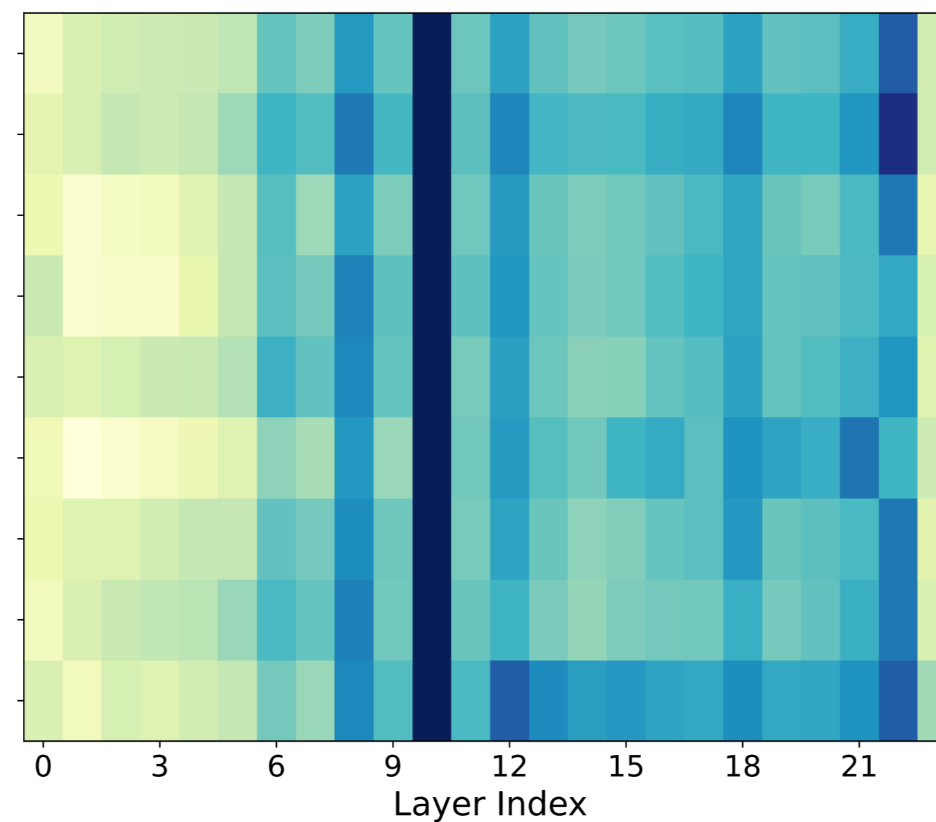
BLOOM-560m (ALiBi)
