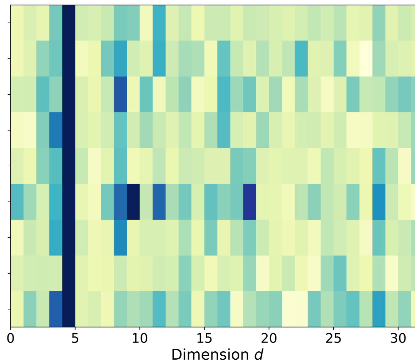
Layer 12, Head 2
