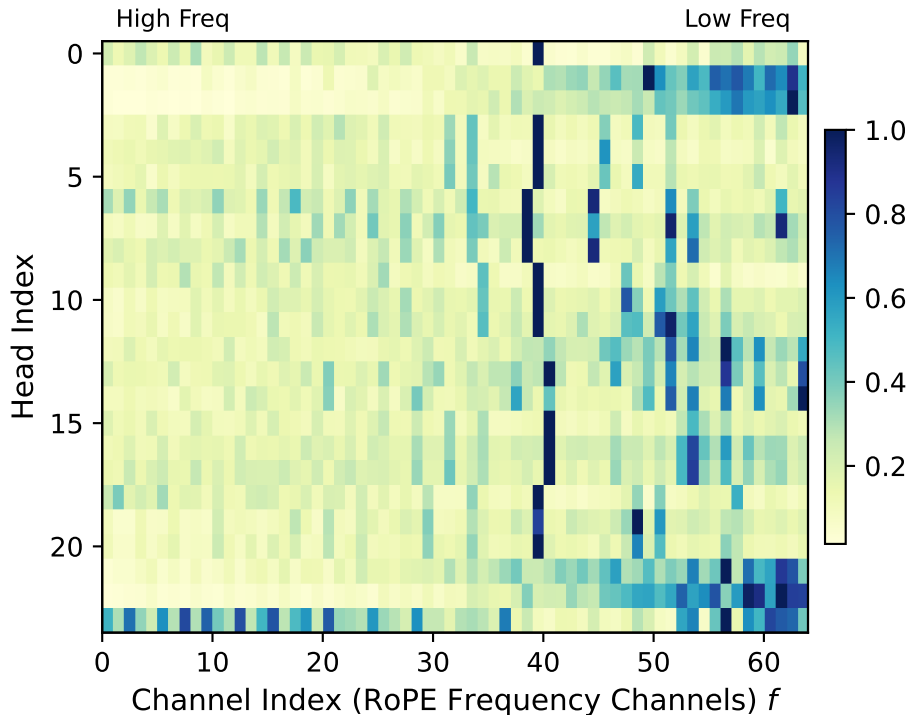
(b) Head-wise Channel Activation (Layer 14)
