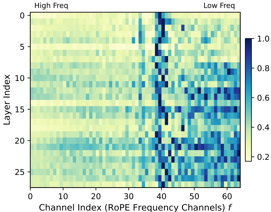
(a) Layer-wise Channel Activation
